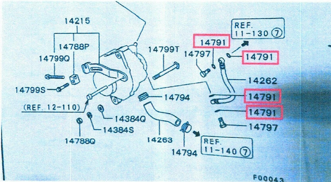
Gambar 5: HOSE ALTERNATOR VACUUM PUMP OIL FEED COPPER WASHER. QTY 04
