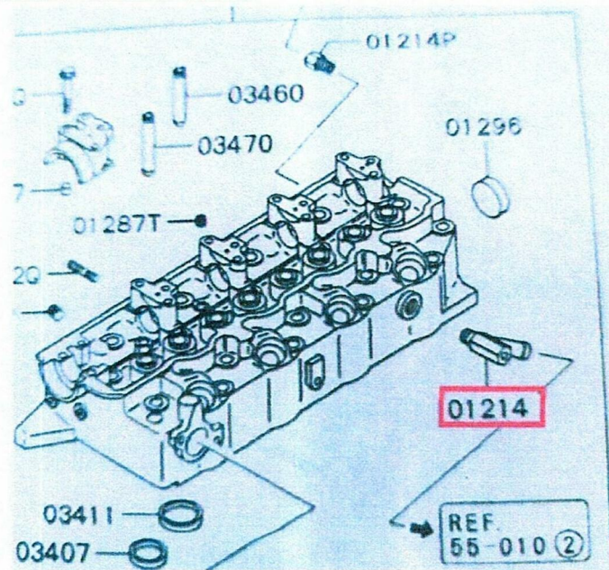
Gambar 9: JOINT, CYLINDER HEAD. QTY:01
