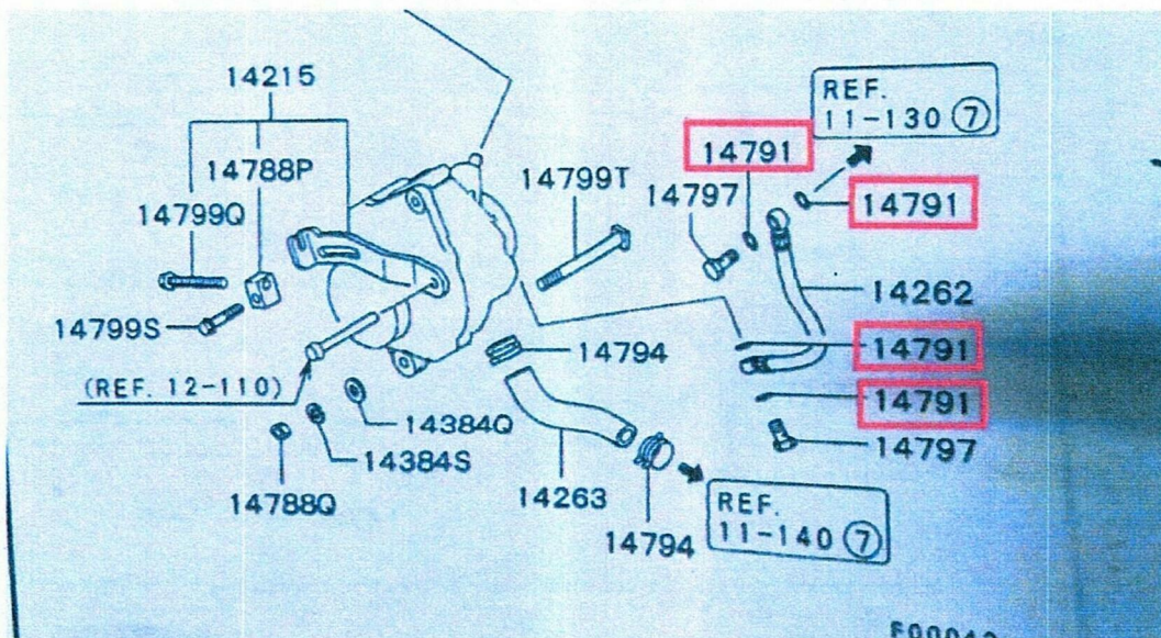
Gambar 10: HOSE ALTERNATOR VACUUM PUMP OIL FEED COPPER WASHER. QTY 04
