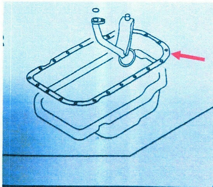
Gambar 2: OIL SUMP GASKET. QTY 01
