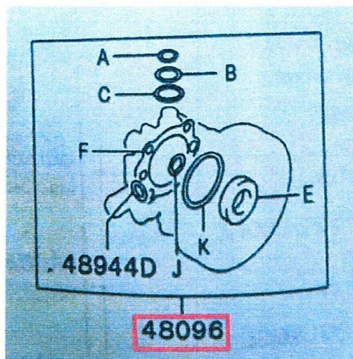
Gambar 11: SEAL KIT, P/s OIL PUMP. QTY 01.
