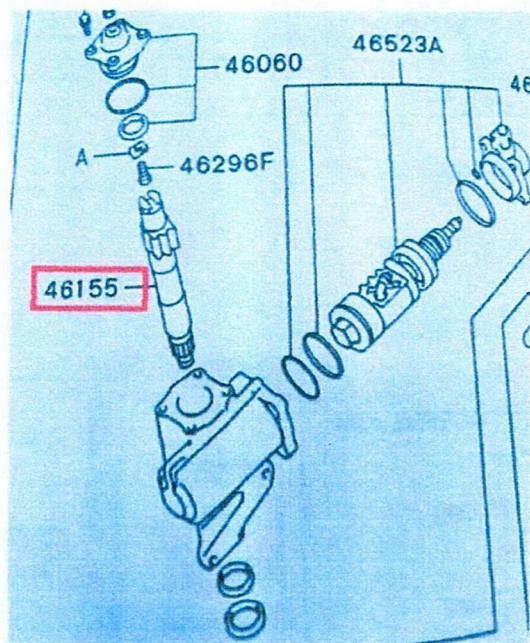
Gambar 13: : SHAFT, STEERING GEAR SECTOR GEAR. QTY 01
