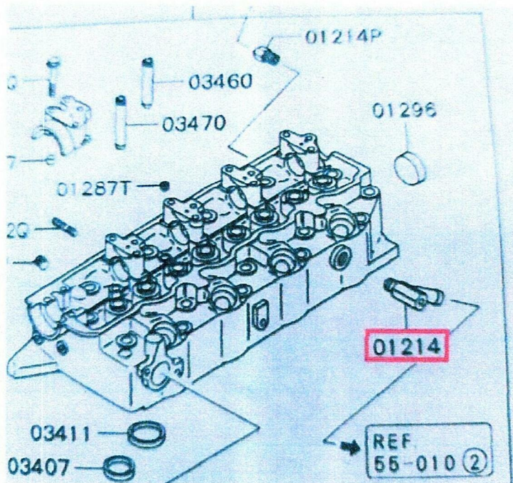
Gambar 6: JOINT, CYLINDER HEAD. QTY:01
