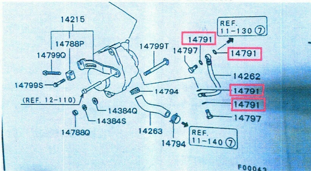
Gambar 1: HOSE ALTERNATOR VACUUM PUMP OIL FEED COPPER WASHER. QTY 04
