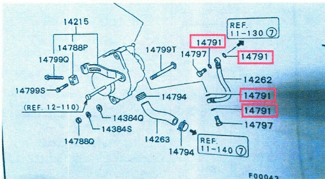
Gambar 3: HOSE ALTERNATOR VACUUM PUMP OIL FEED COPPER WASHER. QTY 04
